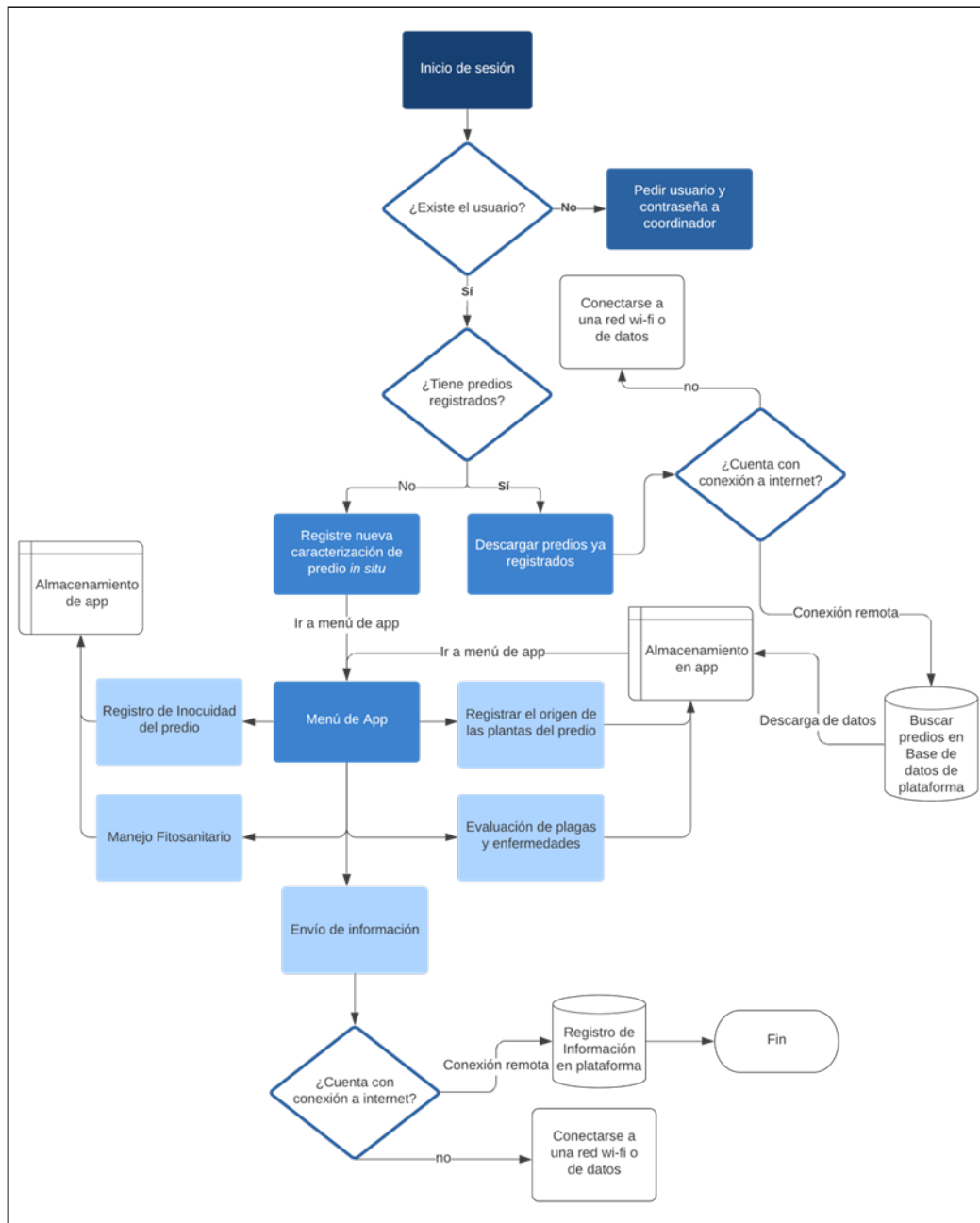
Figure 1. Structural conception flowchart involved during the digital programing of App-ExploraCítricos v2.0 for mobile devices with Android® operating system.
