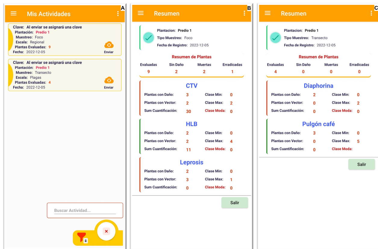
Figure 6. Interface examples of App-ExploraCítricos v2.0 for visualization of assessed farms and consulting reports of phytosanitary assessments in citrus farms. A. 'My Activities' module shows a list and general attributes of assessed farms during day(s). B. Example of a quantitative table 'Report' with records of diseased plants associated to CTV, HLB, and Leprosis for Farm 1 in a 'Focus' sampling type. C. Example of a 'Report' with records of plants infested associated to pests 'Diaphorina' ( D. citri ) and 'Pulgón café' ( T. citricida ). The vector category is only selected if the respective pathogen has been confirmed by diagnostic in the sampling region.
